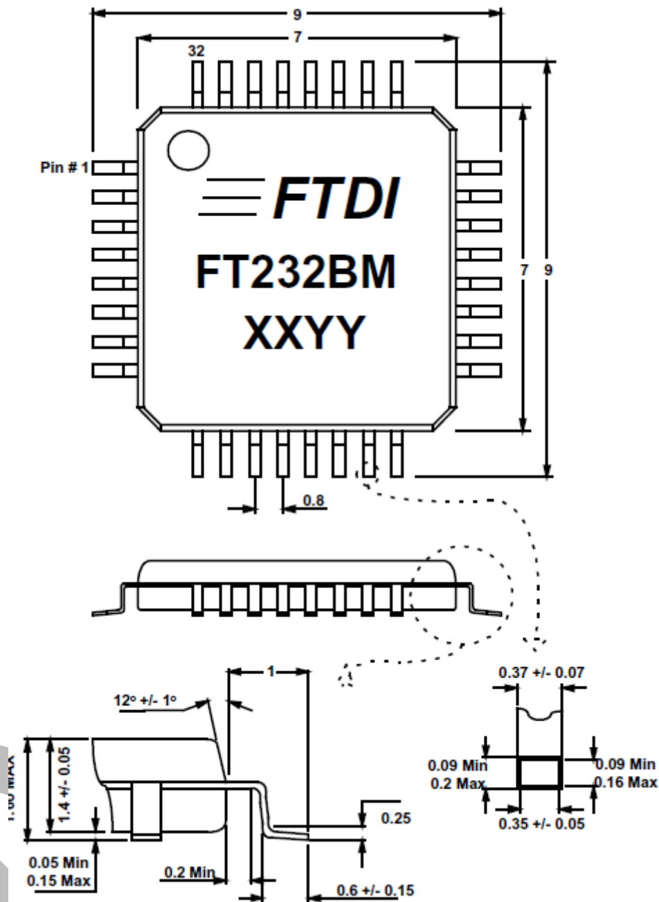
Figure 10.1 32 LQFP Package Dimensions
